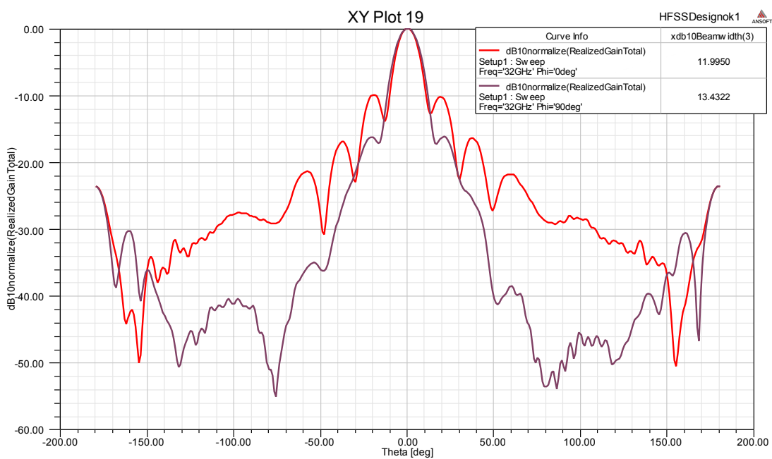
Gain@32GHz
