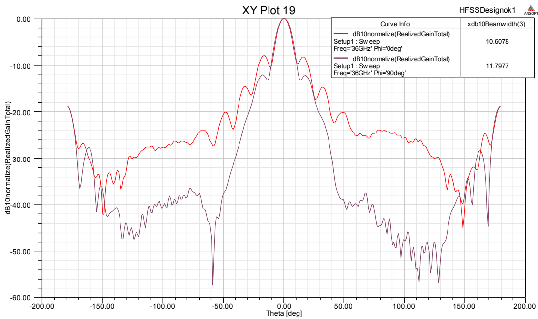
Gain@36GHz
