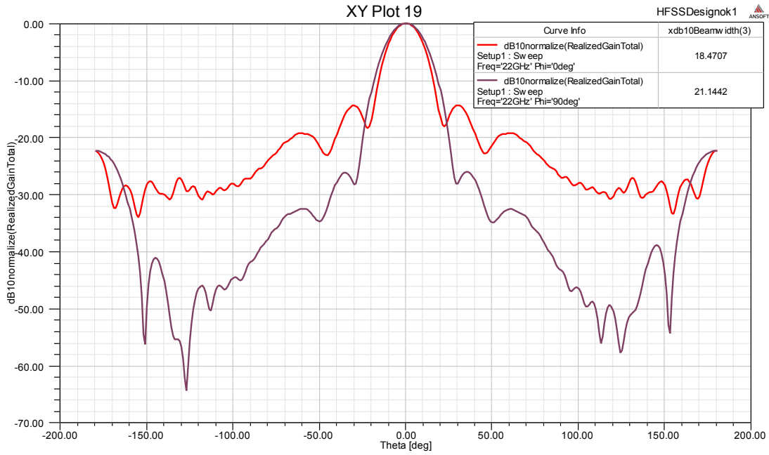
Gain@22GHz
