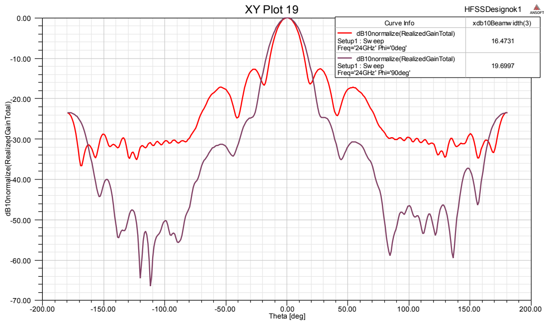
Gain@24GHz
