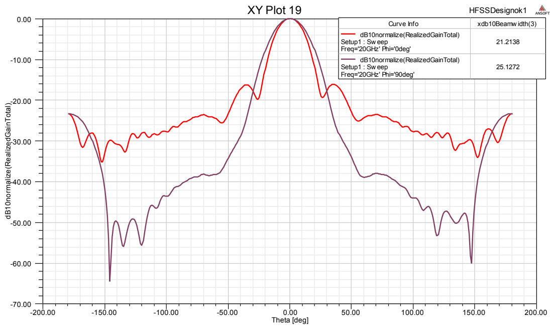
Gain@20GHz
