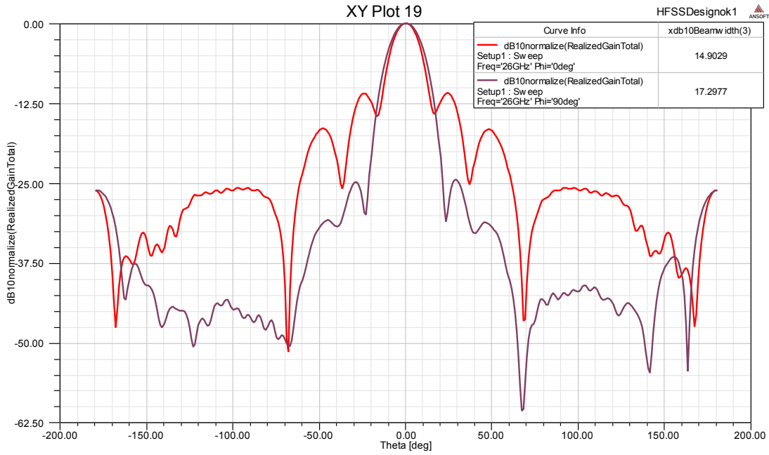
Gain@26GHz
