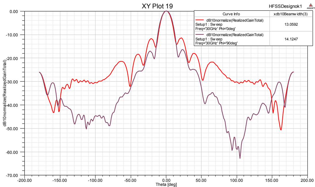
Gain@30GHz
