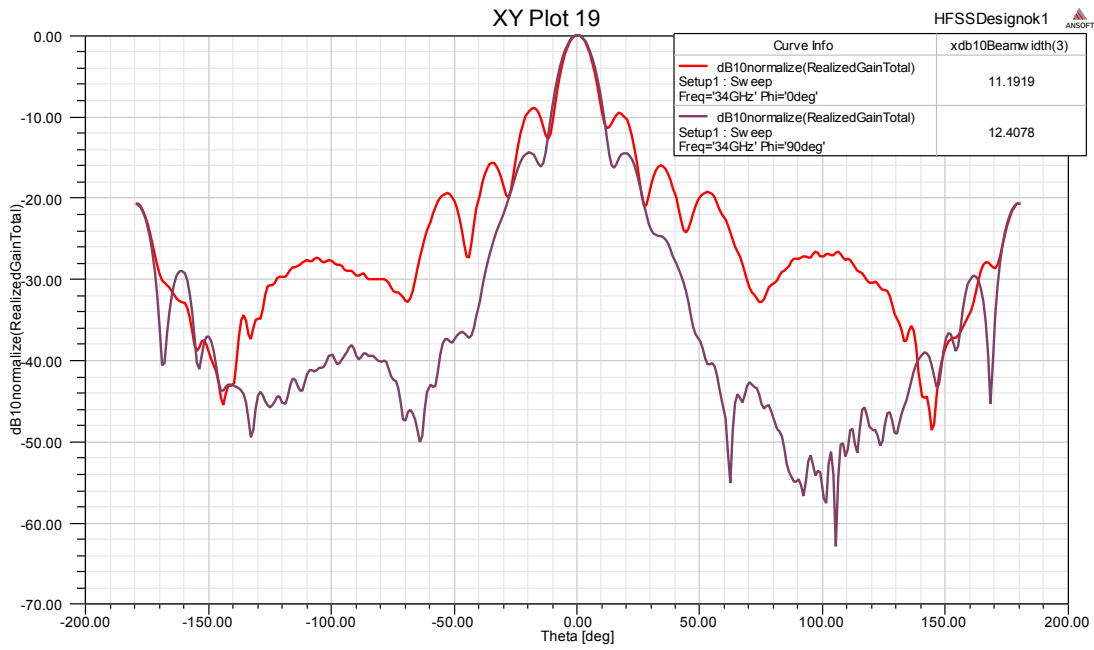
Gain@34GHz
