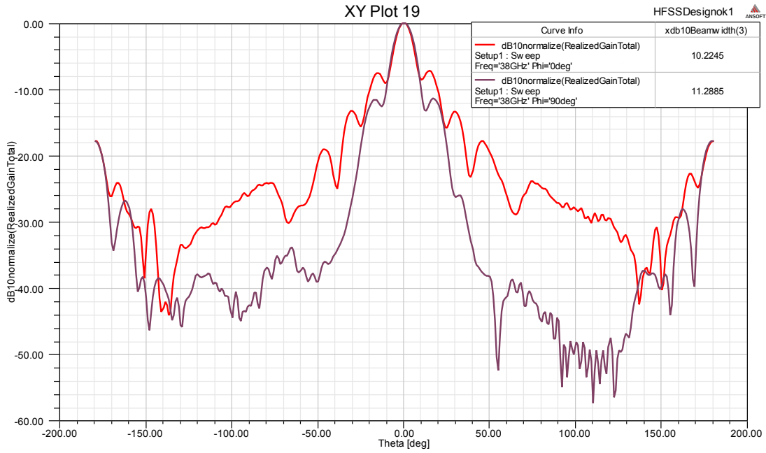
Gain@38GHz
