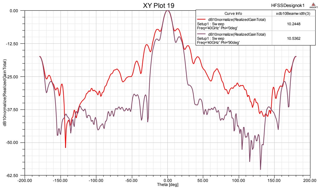
Gain@40GHz
